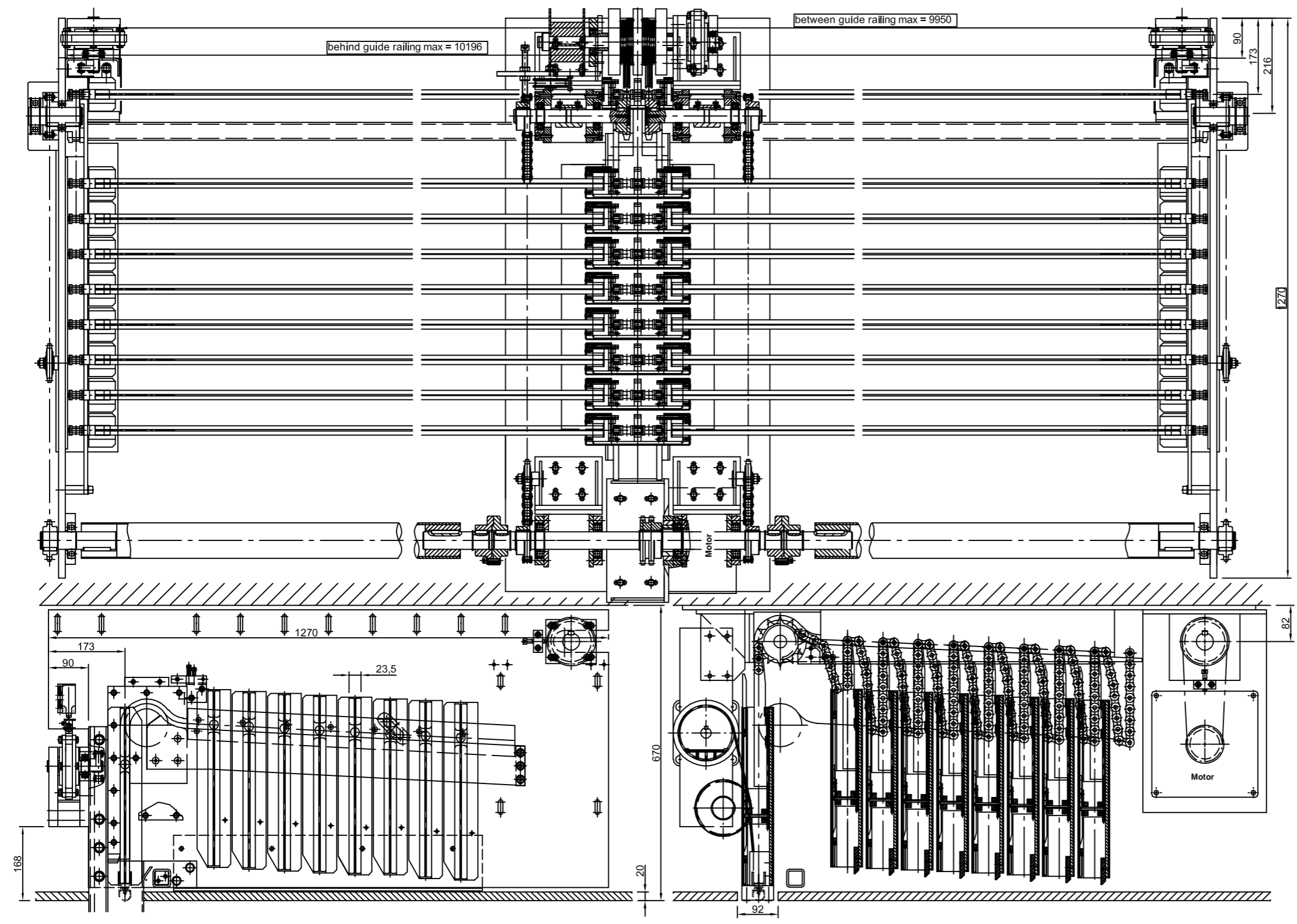
Drive train 2x GG/2-398, 9 panels Dimensions in mm Scale 1:10
